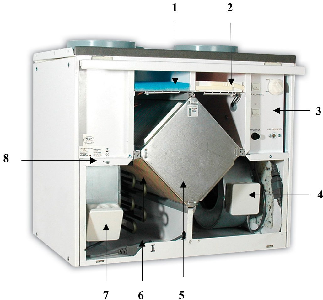
ECO 130S R
